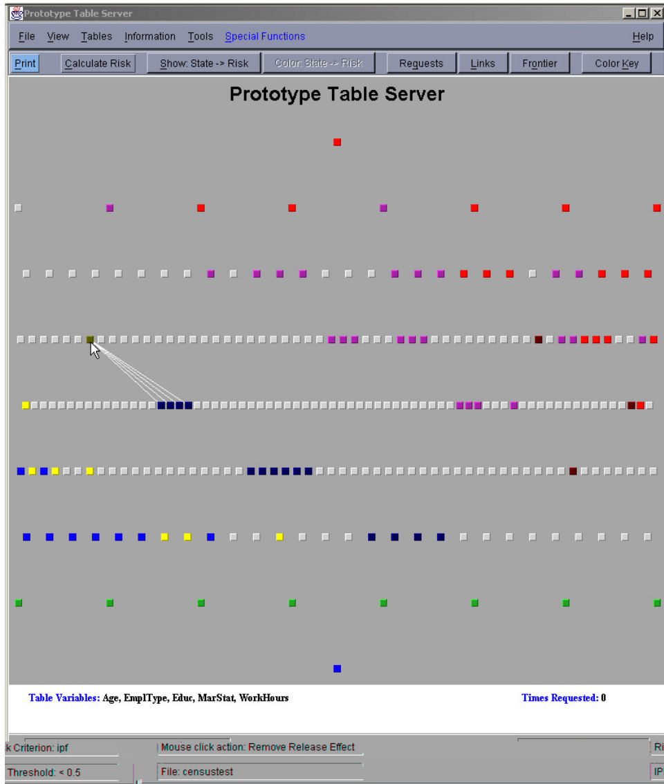
Figure 2: Visualization of the query space for a table server operating on an 8-dimensional table. The risk criterion is the accuracy with which the full table can be reconstructed using iterative proportional fitting (see §2.1.4). Shown are the previous releases (yellow and blue), core releases made when the system begins operation (green), and tables that are already too risky (red). The cursor highlights a particular proposed release. Releasing this table would, however, render all magenta and brown tables (one of which is even three-dimensional) unreleasable in the future.
