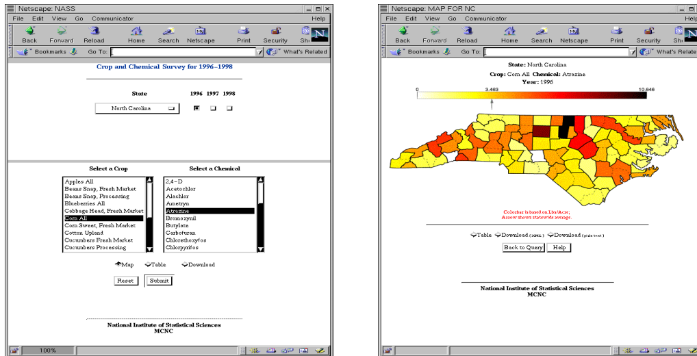
Figure 1: Input-screen (left): Users first select the State from which the data are required. Next, they select a crop (or chemical) from the menu. Then, the adjacent menu is regenerated to contain only the chemicals (or crops) associated with the selected crop or chemical. Year(s) and output formats may be specified at any time before submitting the query. Output Screen (right): The map displays the pounds per acre of Atrazine used on Corn for all (super)counties in North Carolina in 1996 , using artificial data. The color key shows the numerical values, with a marker indicating the statewide average usage. The display allows users to identify both individual counties and parent supercounties.
